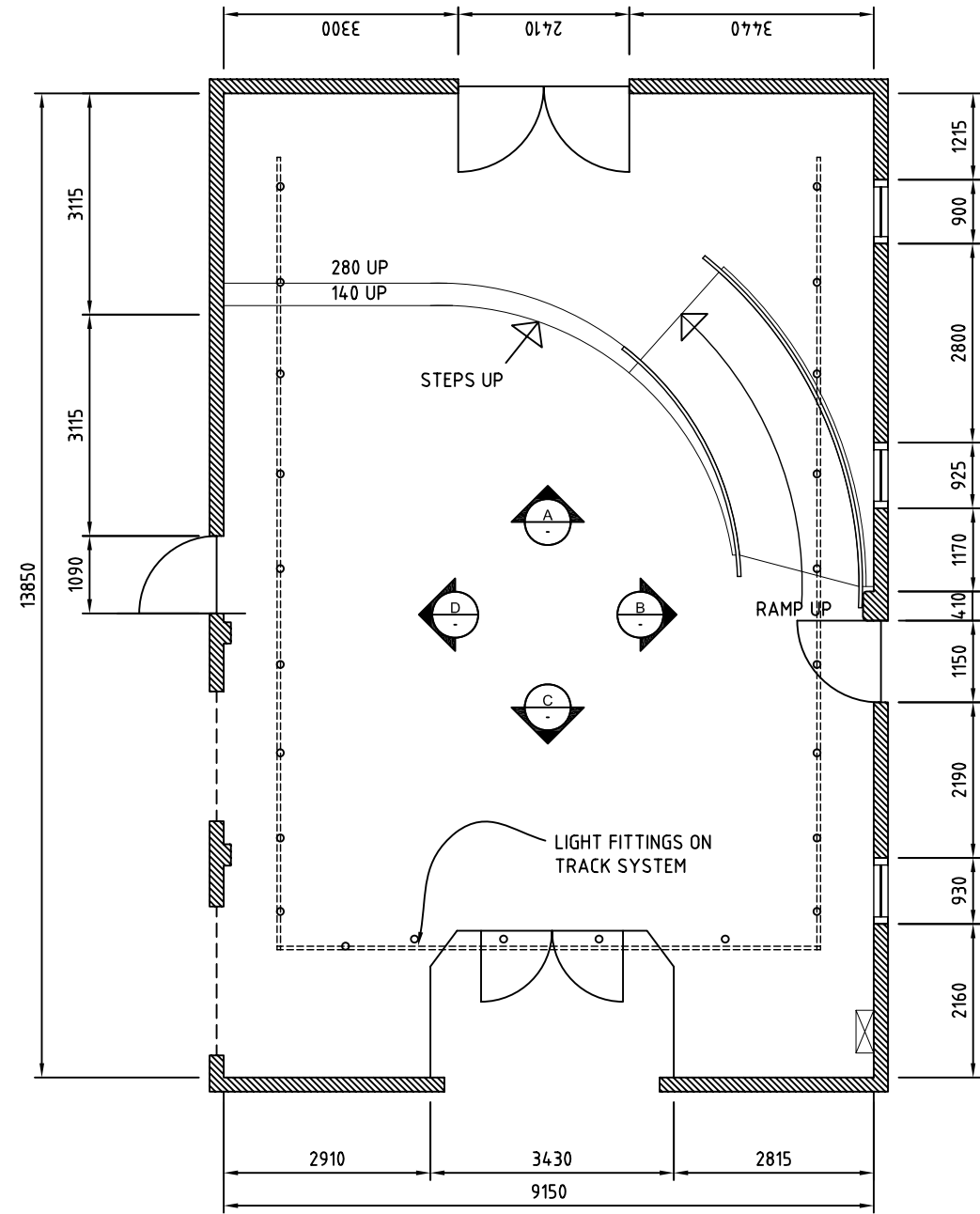
1 PLAN SCALE 1:100
