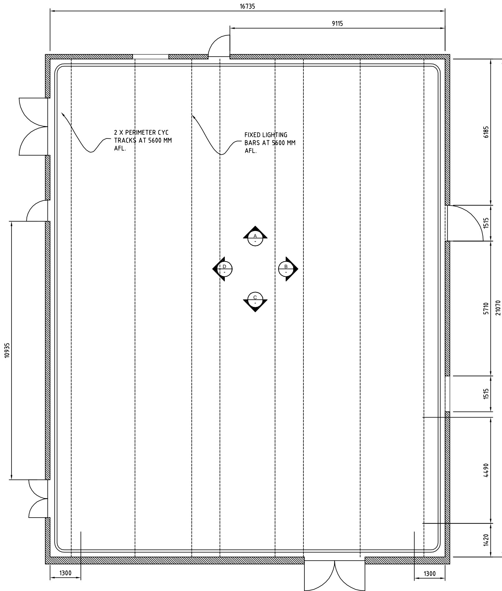
1 PLAN SCALE 1:100
