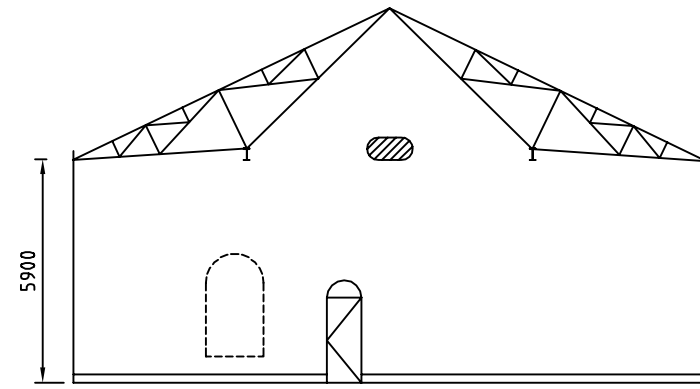
A ELEVATION SCALE 1:200
