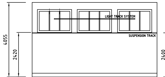
C ELEVATION SCALE 1:100
