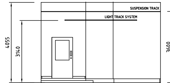
B ELEVATION SCALE 1:100
